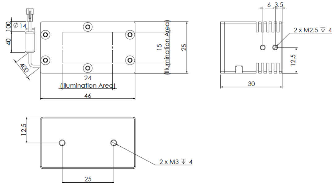
Lighting Dimension
